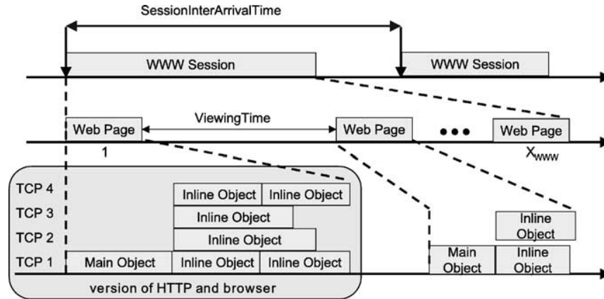
Figure 3. Source model for WWW traffic.
