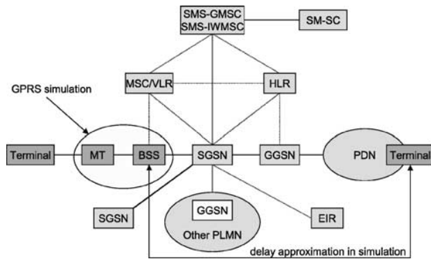
Figure 7. Overview of the GPRS logical architecture.
