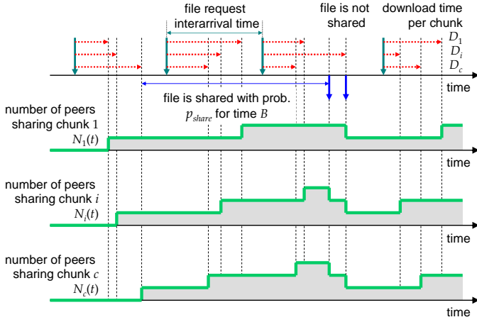
Fig. 3. Arrival process of peers sharing chunks of a file
