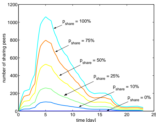
Fig. 11. Number of sharing peers depending on the file sharing probability
