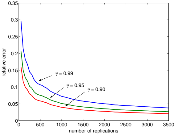
Fig. 7. Relative error in dependence of the number of replications
