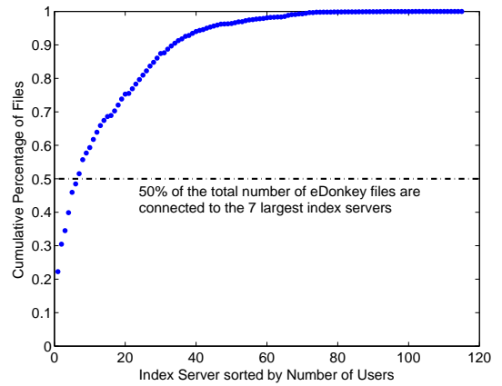
Fig. 1. Number of users connected to different index servers
