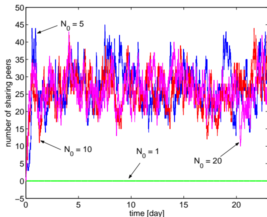
Fig. 14. Influence of the number of initially sharing peers
