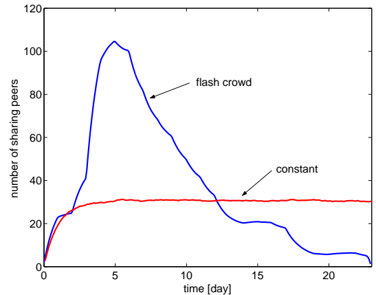
Fig. 9. Number of sharing peers for flash crowd and constant behavior
