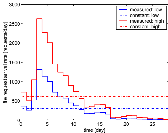
Fig. 6. File request arrival rates of the nonstationary Poisson process
