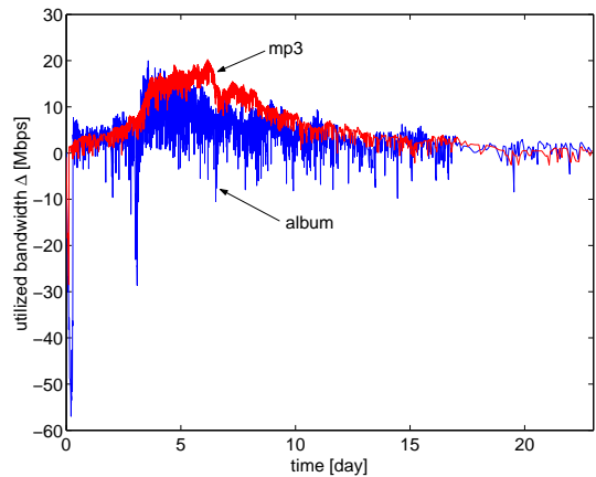
Fig. 12. Utilized bandwidth for an mp3-audio file and an entire album
