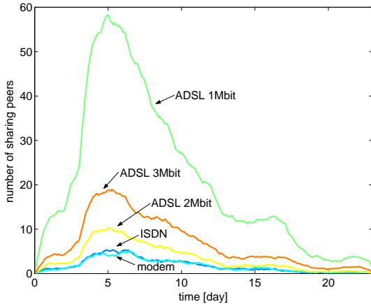
Fig. 10. Number of sharing peers in dependence of the access bandwidth
