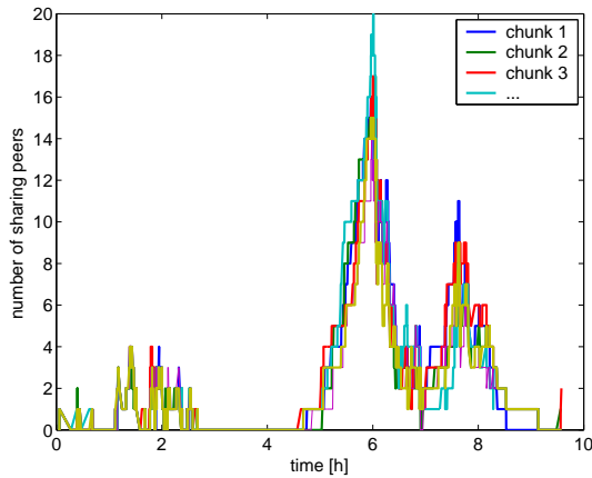
Fig. 5. Detailed simulation of the eDonkey specific mechanisms
