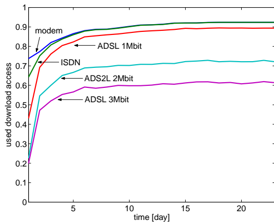
Fig. 13. Used download bandwidth over time
