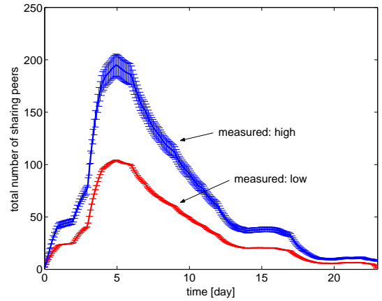
Fig. 8. Number of sharing peers for measured arrival rates
