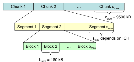
Fig. 2. Structure of a file on eDonkey application layer
