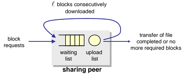
Fig. 4. Upload queue model
