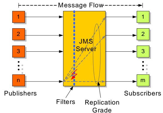
Figure 1: The JMS server decouples publishers and subscribers.
