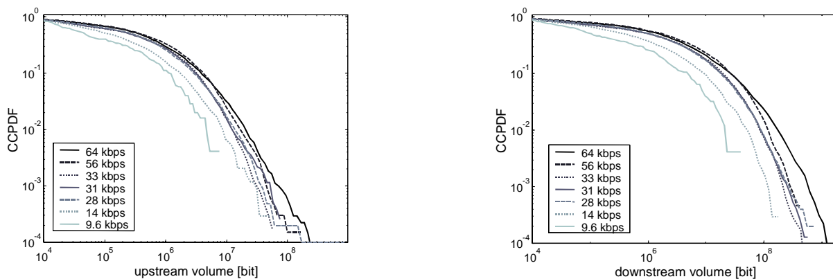
Figure 5: Session up- and downstream volume distribution.
