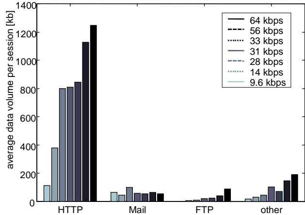
Figure 6: Average data volume per service (HTTP, Mail, FTP) and session.
