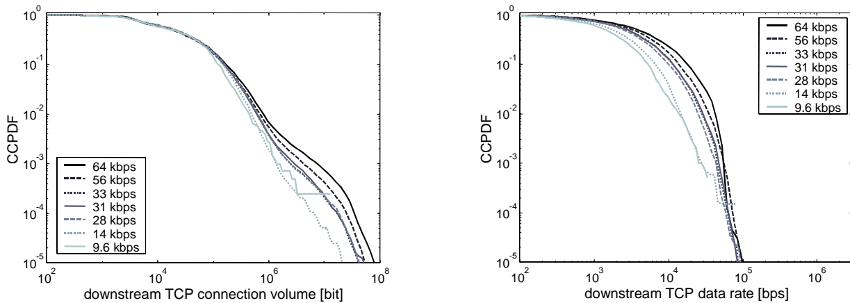
Figure 8: TCP-connection volume (left) and TCP data rate (right) distribution.
