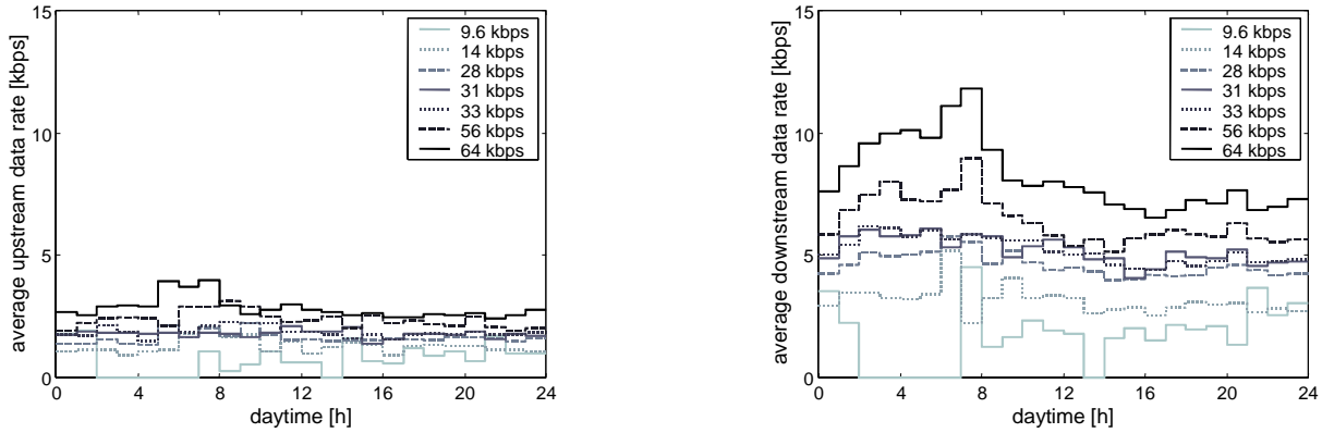
Figure 7: TCP-connection data rate in dependence of daytime.
