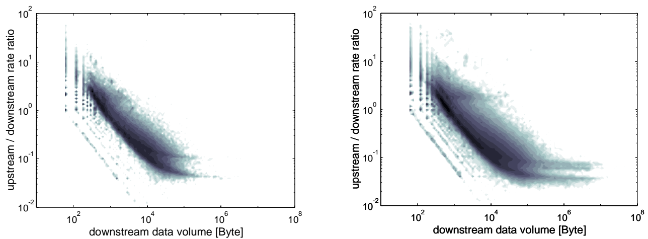
Figure 10: TCP data rate ratio in dependence of downstream data volume for 14.4kbps(left) and 64kbps (right).
