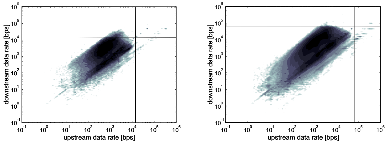
Figure 9: TCP data rate correlation for 14.4kbps (left) and 64kbps (right).
