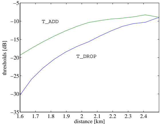
Figure 5: Soft-handoff thresholds depending on the inter-BS distance ( \lambda = 3 )
