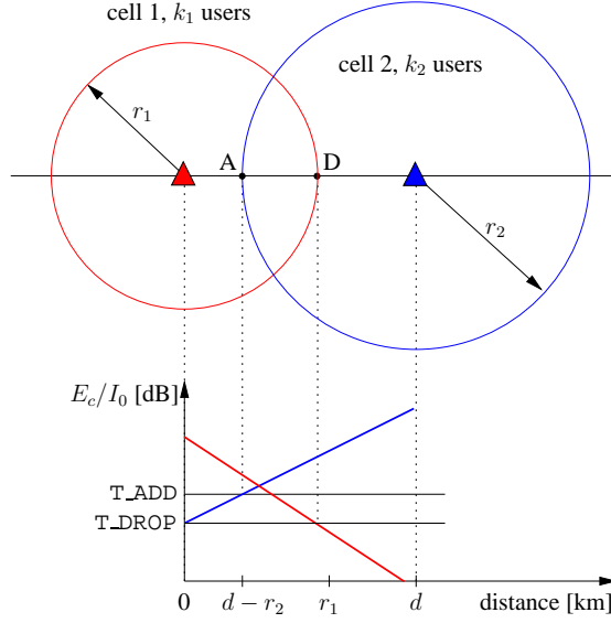
Figure 4: Variations of soft-handoff thresholds due to fluctuations of traffic
