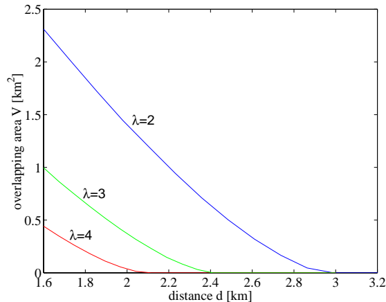
Figure 7: Minimum soft-handoff region for different traffic intensities
