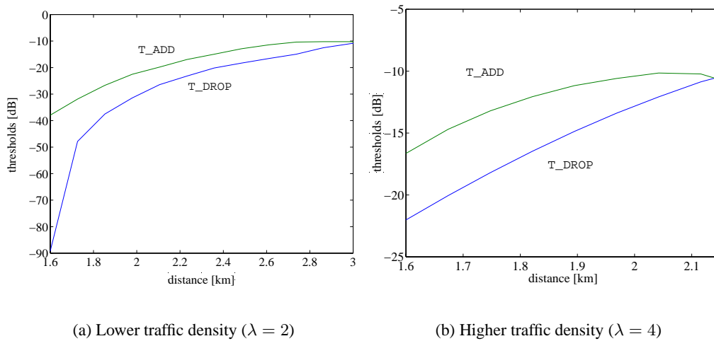
Figure 6: Soft-handoff thresholds depending on inter-BS distances
