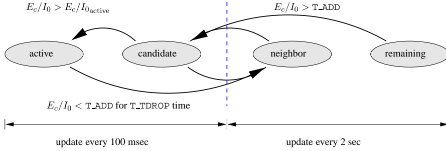
Figure 1: Soft-handoff set maintenance
