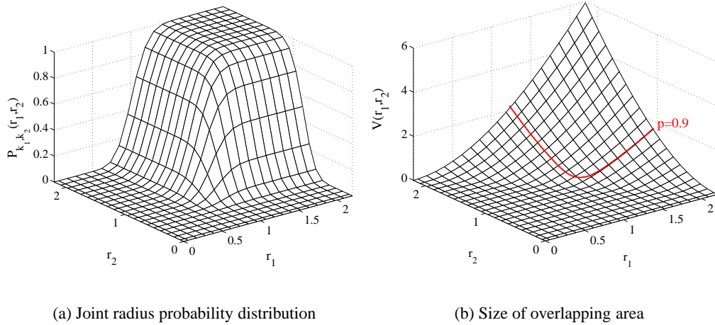
Figure 2: Radius distribution and overlapping area
