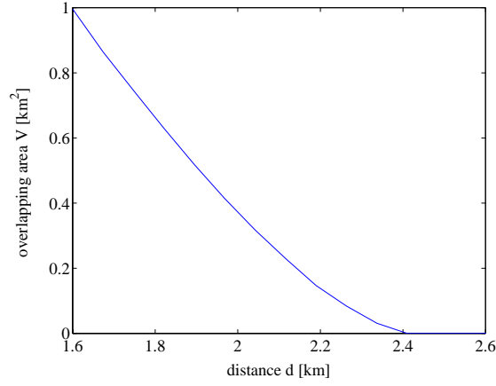
Figure 3: Minimum overlapping area according to inter-BS distance
